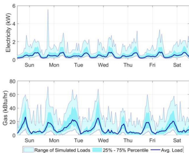
Fig. 13. The range of electricity and natural gas loads captured in the single-family BEM workflow during a winter week. The figure shows the average load across all single-family buildings, the range of loads captured between the 25th and 75th percentile during each time step, and the complete range single-family simulation results.
