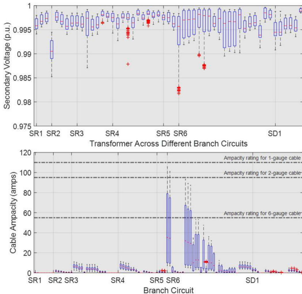
Fig. 15. Per unit secondary voltage distribution and line ampacity across all nodes, transformer and, cables in the Oak View Community ACPF.
