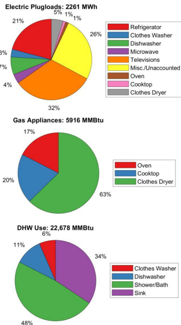
Fig. 14. Pie charts showing end use breakdowns for annual energy use in the residential sector. Results are shown for electric and natural gas use. Since DHW loads have a large impact on community wide energy use, natural gas results are split between gas appliances and DHW use. Gas space heating, which is not pictured here, uses 4,602 MMBtu per year across all residential buildings.
