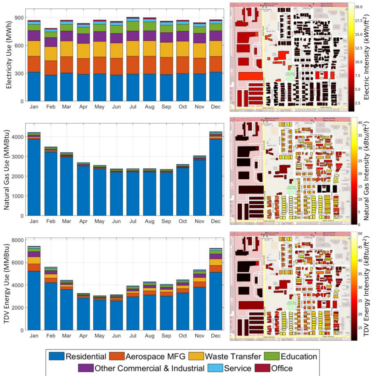
Fig. 11. Modeled community scale energy use broken down by month and building type. Corresponding maps show the modeled annual EUI for each building type, showing where and how energy is being used in the community. Results are presented for total electricity use, natural gas use, and TDV energy use.
